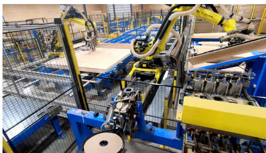
Paradigm Panel – Robotic framing line
